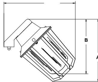
STANCHION MOUNT
